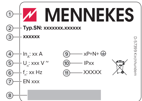
Fig. 1: Rating plate (example)
