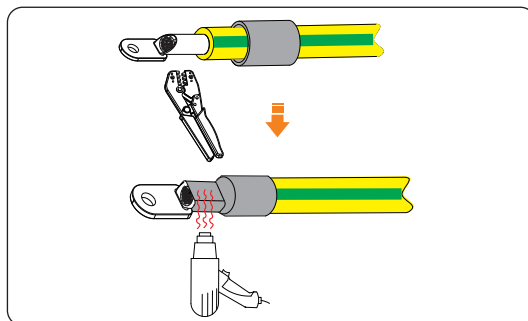
Figure 7-5 Crimping and heating
