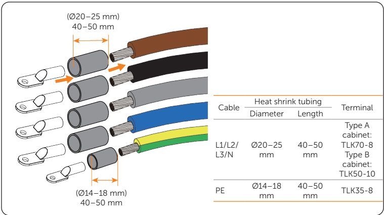
Figure 7-8 Attaching tubing and ring terminals
