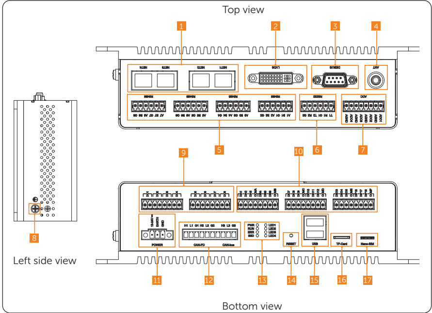
Figure 2-13 Appearance of the EMS
