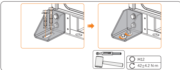
Figure 6-9 Tightening expansion bolts
