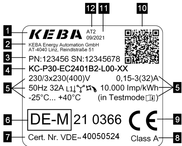
Fig. 3-2: Type plate (example)
